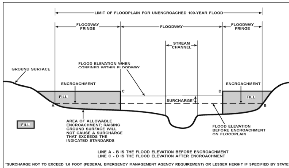
FIGURE 1 – FLOODWAY SCHEMATIC
